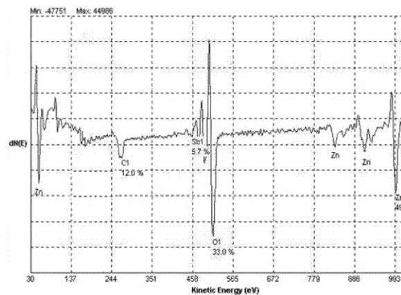
Figure 2. Auger survey for ZnO:Sb thin films
