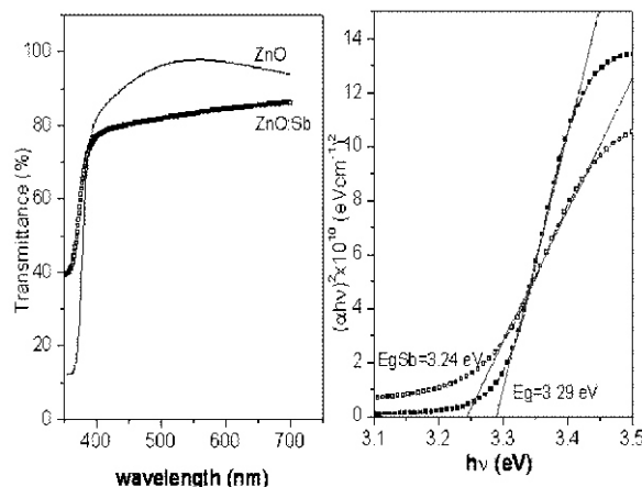
Figure 4. (a) Transmittance spectra (b) Evaluation of E_g for ZnO and ZnO:Sb thin films
